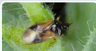
Orius sp.
